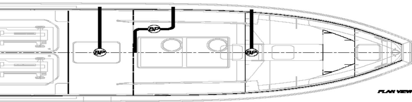
FWD & AFT BILGE PUMPS
